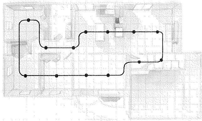
AQUASAFE Looped System: Each sprinkler is connected to a main line loop of ¾" or 1" tubing.
